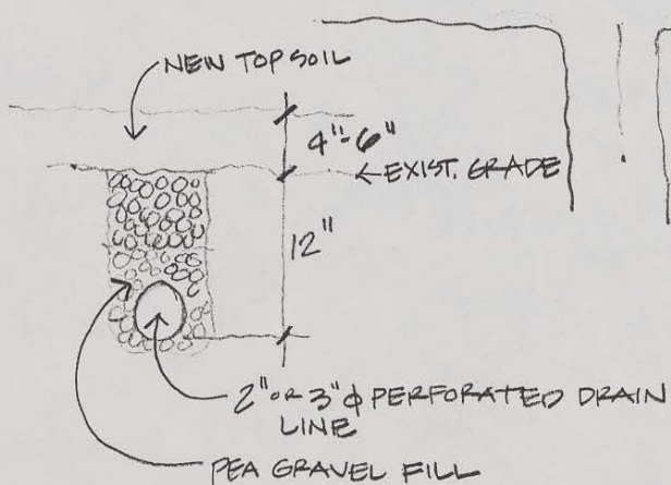
3A TYPICAL SECTION THRU DRAIN LINE
